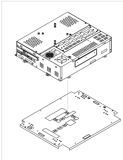
FIGURE 5-6: LCD MODULE TO MAIN SYSTEM
