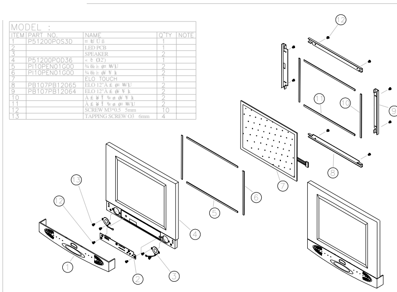
FIGURE 5-2: DISPLAY PAC-PPC 12.1" FRONT BEZEL
