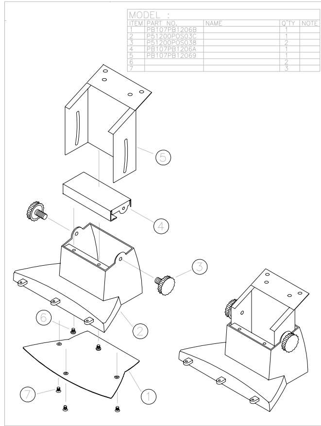
FIGURE 3-3: DISPLAY PAC-PPCSMALL BASE ASSEMBLY
