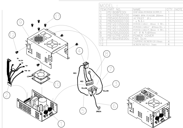
FIGURE 5-7: DISPLAY PAC-PPCAC POWER MODULE
