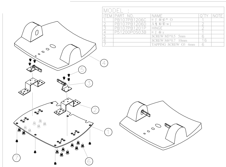
FIGURE 3-2: BIG PEDESTAL ASSEMBLY
