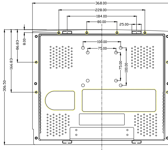
FIGURE 3-13: DISPLAY PAC-PPC 12.1" VESA
