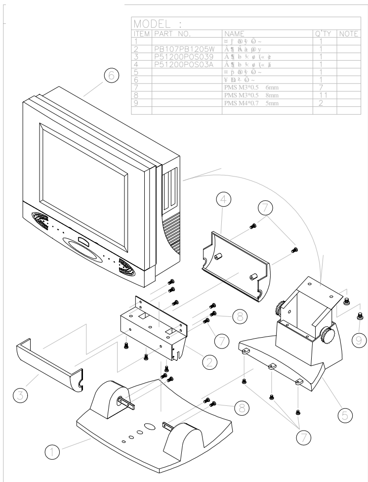
FIGURE 3-1: DISPLAY PAC-PPCSTAND A
