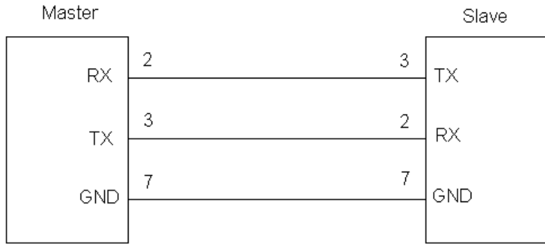
Figure 9-2. RS232 Wiring Diagram
