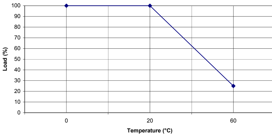
Temperature Derating
