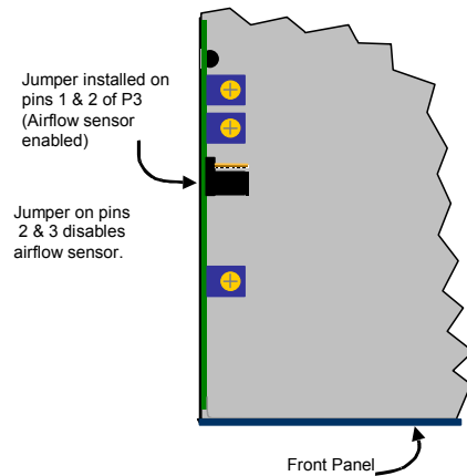
Location of Airflow Sensor Jumper – Top View
